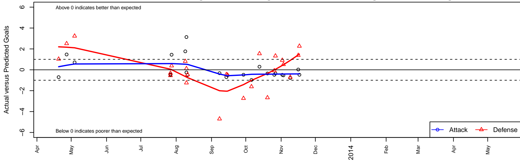
3 Rivers Black B98 Dots are actual minus expected GF (blue circles) and GA (red triangles). Blue line is smoothed change in attack strength. Red is smoothed change in defense strength.
